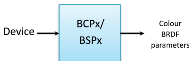
Figure G.5 — BRDF parameters from profile with chromatic BRDF tags
