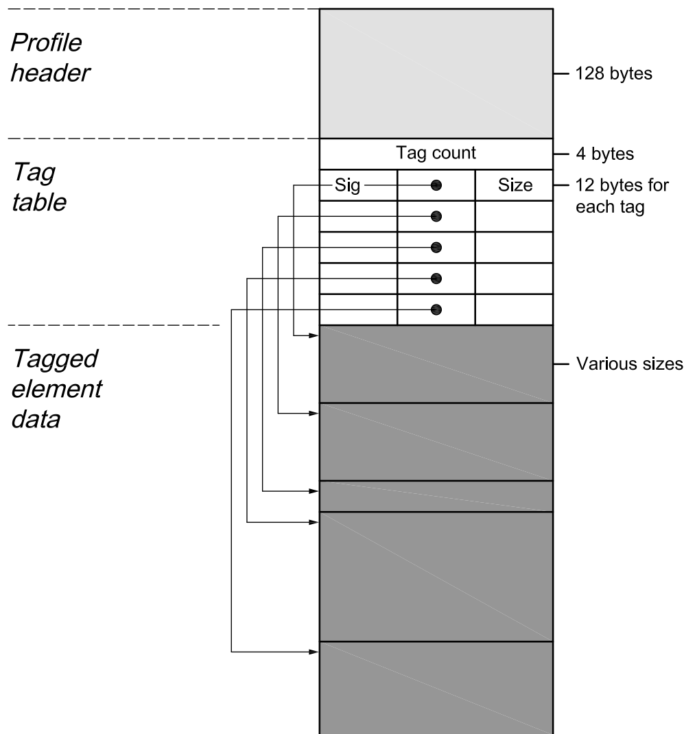
Figure 6 — Profile structure
